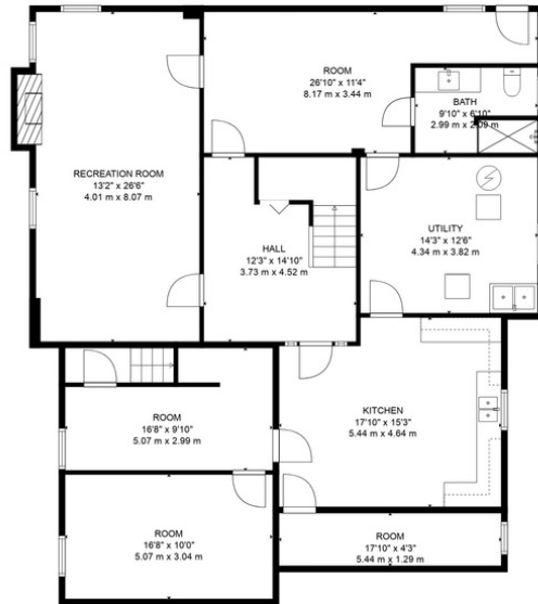
FLOOR 1
