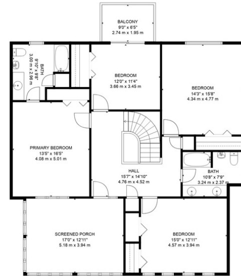
FLOOR 3
