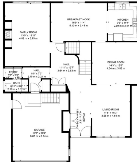
FLOOR 2
