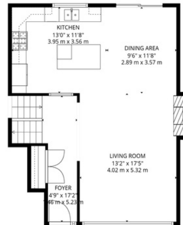
FLOOR 3
